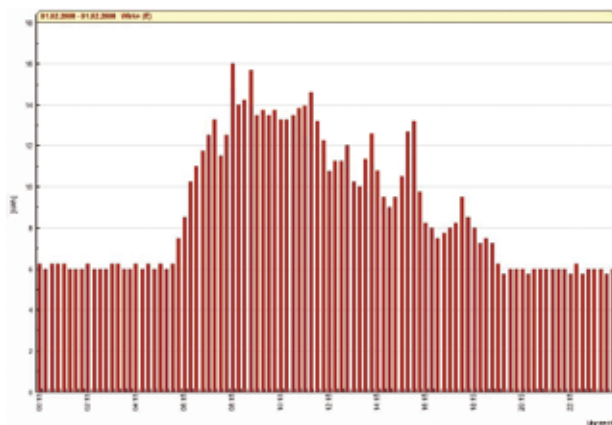
Suboptimaler Lastgang
